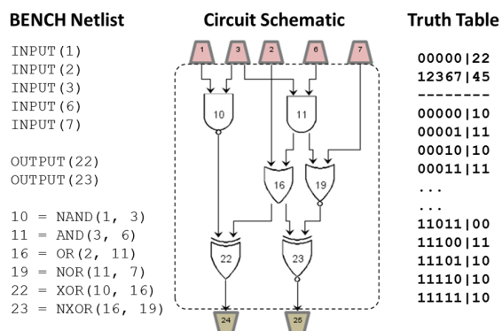
Figure 2: Equivalent Circuit Representations
