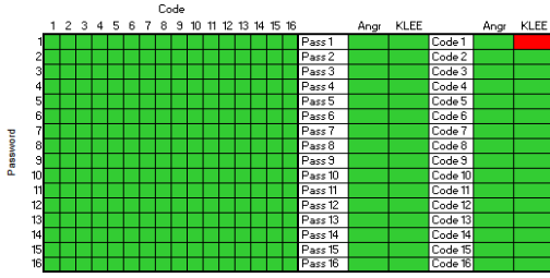
Figure 8: SBHA Effectiveness against Angr/KLEE
