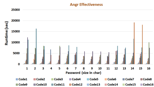
Figure 7: Tigress Pass/Code Combined Benchmarks analysis
